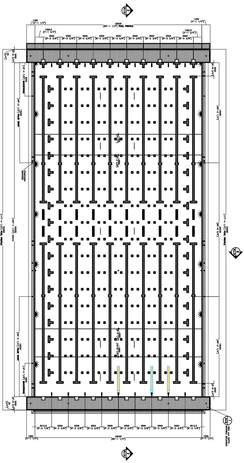
2 50m COMPETITION POOL MOVABLE BALUNZO LOCATIONS SCALE 1:100
